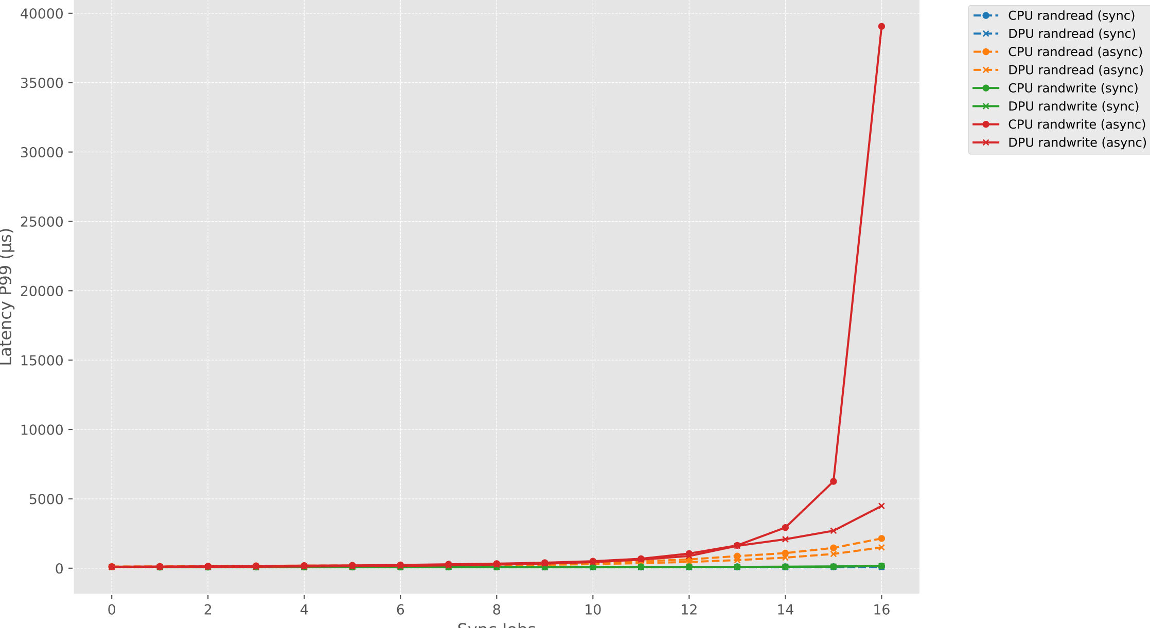
Latency P99 vs Sync Jobs (async1 syncN) - RAND (CPU vs DPU)
